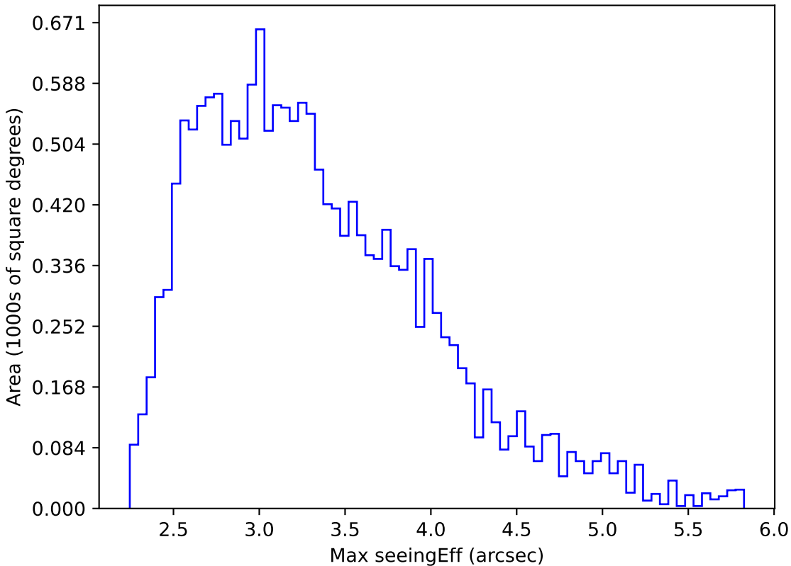
too_elab_r8_d3_ugrizy_v3.4_10yrs WFD all bands: Max seeingEff
