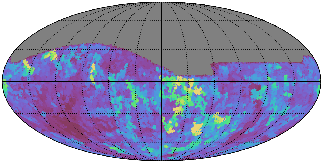
too_elab_r8_d3_ugrizy_v3.4_10yrs All sky z band: Max seeingEff
