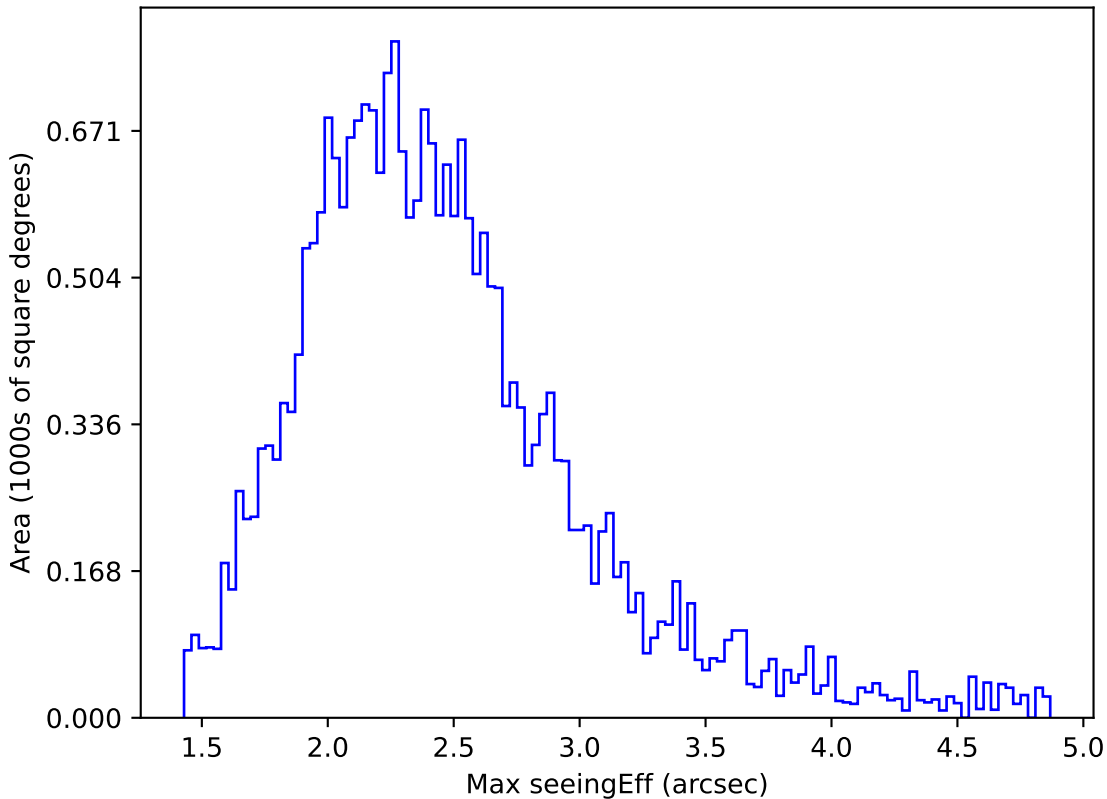
too_elab_r8_d3_ugrizy_v3.4_10yrs All sky z band: Max seeingEff
