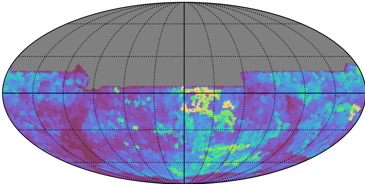
too_elab_r8_d3_ugrizy_v3.4_10yrs All sky y band: Max seeingEff
