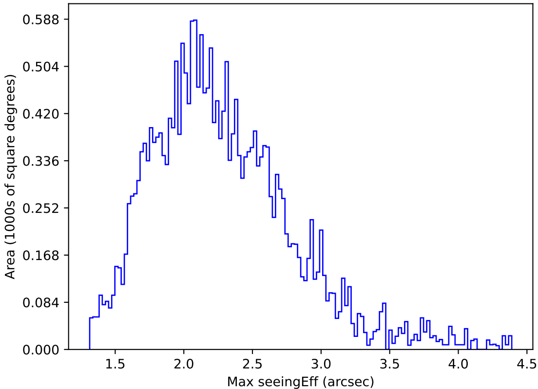
too_elab_r8_d3_ugrizy_v3.4_10yrs All sky y band: Max seeingEff
