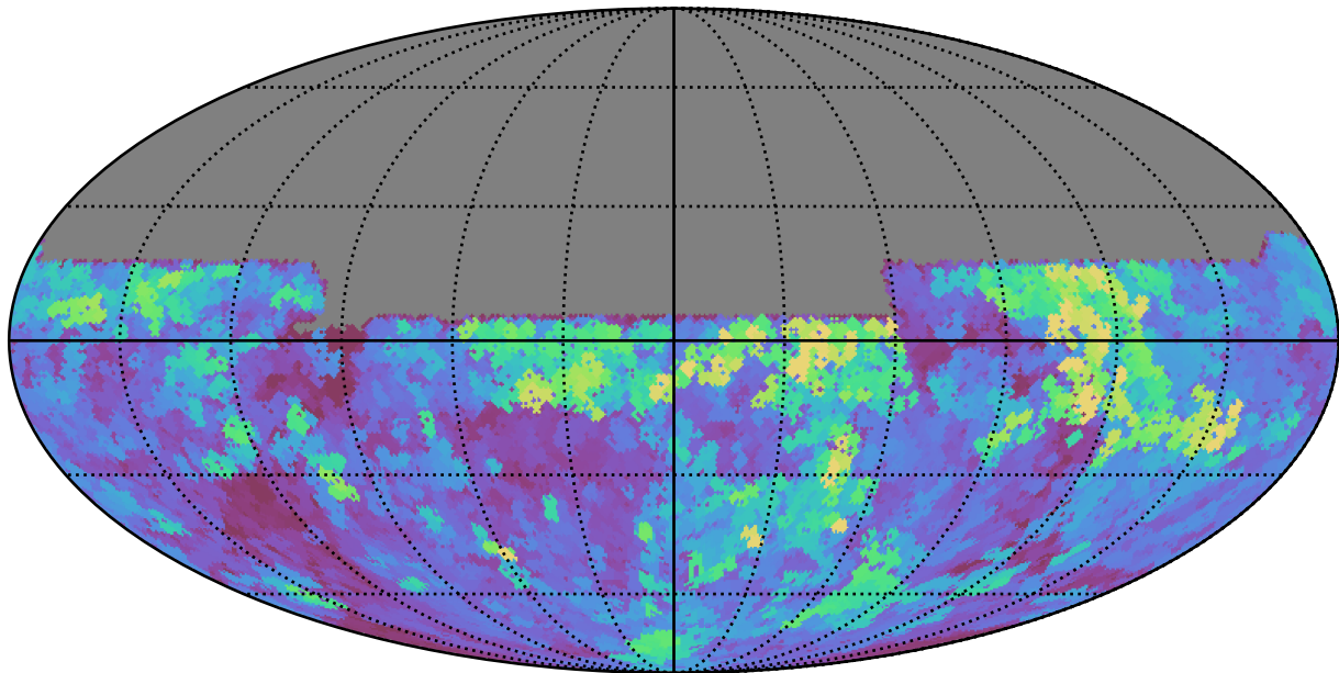
too_elab_r8_d3_ugrizy_v3.4_10yrs All sky u band: Max seeingEff
