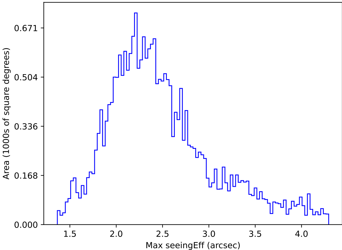
too_elab_r8_d3_ugrizy_v3.4_10yrs All sky u band: Max seeingEff
