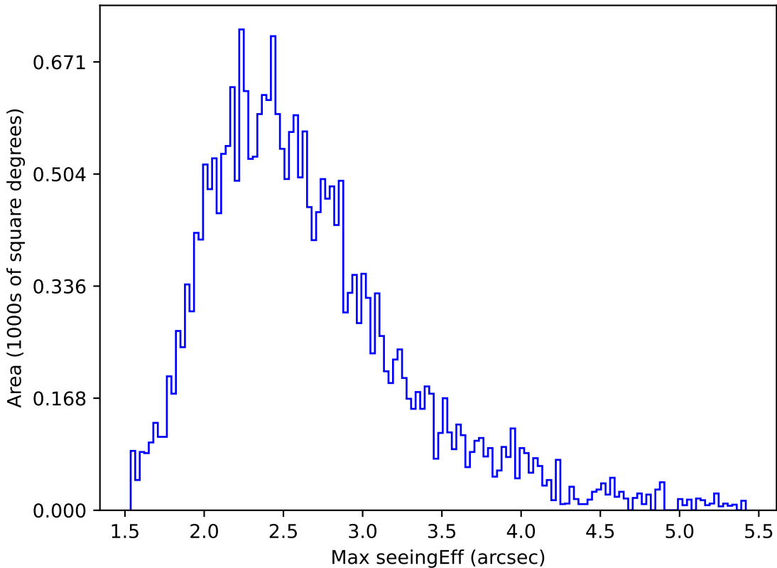
too_elab_r8_d3_ugrizy_v3.4_10yrs All sky r band: Max seeingEff
