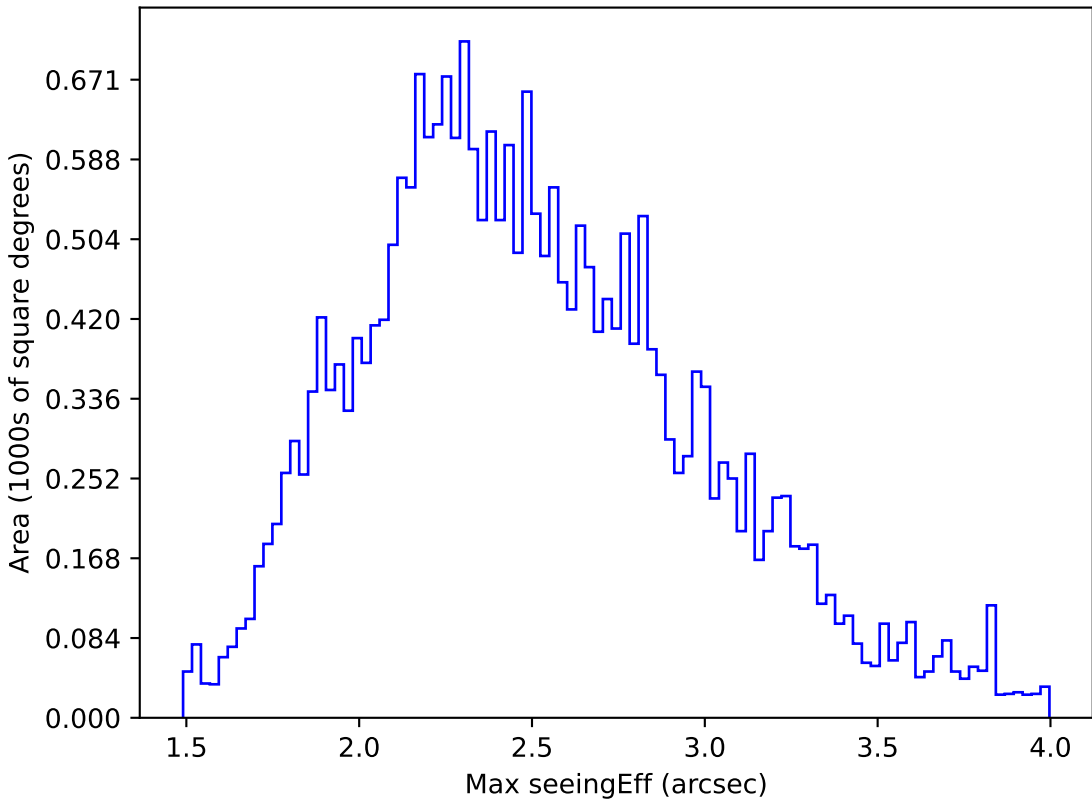
too_elab_r8_d3_ugrizy_v3.4_10yrs All sky g band: Max seeingEff
