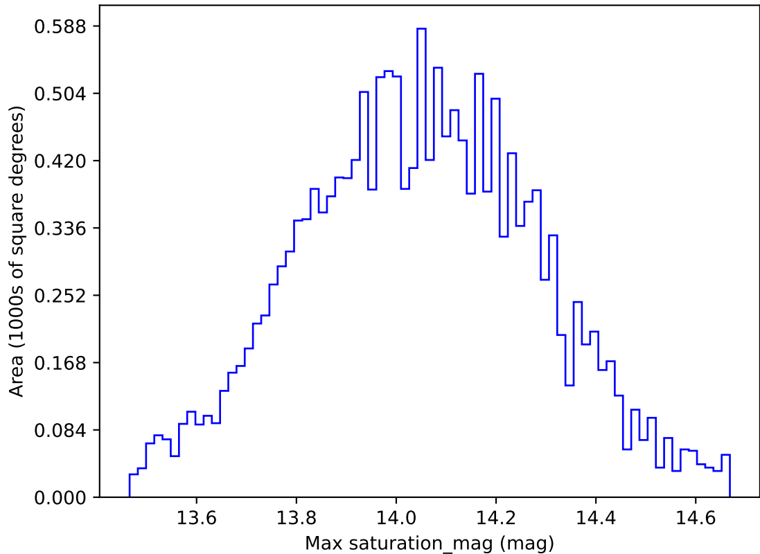
too_elab_r8_d3_ugrizy_v3.4_10yrs WFD u band: Max saturation_mag
