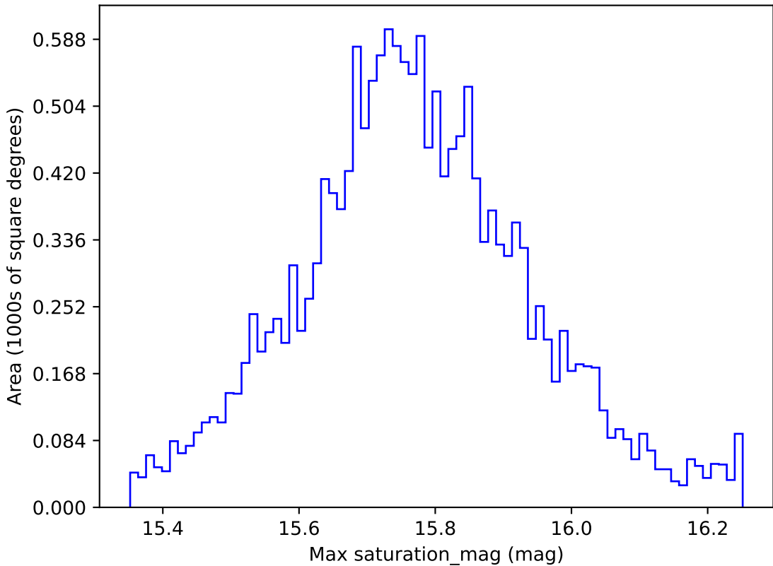
too_elab_r8_d3_ugrizy_v3.4_10yrs WFD r band: Max saturation_mag
