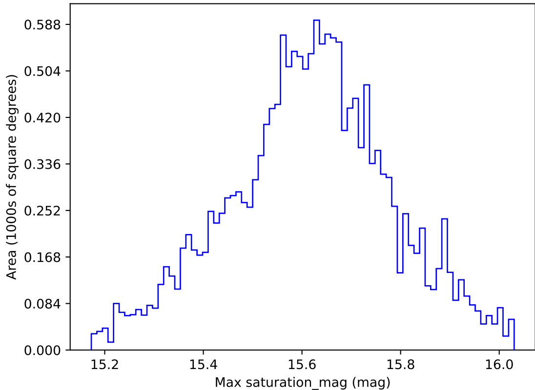
too_elab_r8_d3_ugrizy_v3.4_10yrs WFD i band: Max saturation_mag
