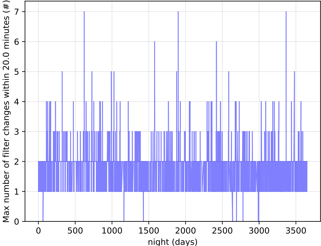
too_elab_r8_d3_ugrizy_v3.4_10yrs Per Night: Max number of filter changes within 20.0 minutes
