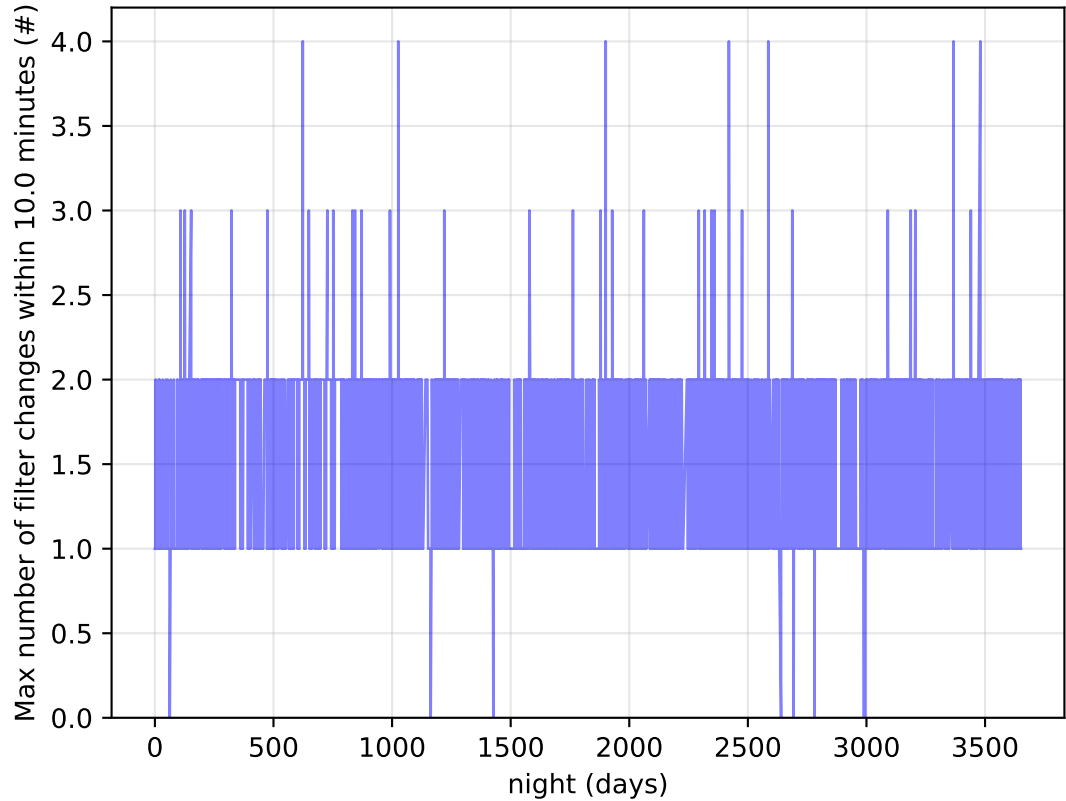
too_elab_r8_d3_ugrizy_v3.4_10yrs Per Night: Max number of filter changes within 10.0 minutes
