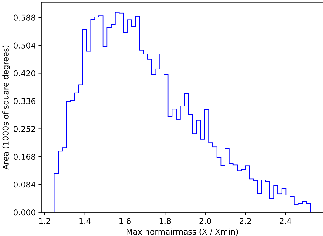
too_elab_r8_d3_ugrizy_v3.4_10yrs WFD u band: Max normairmass
