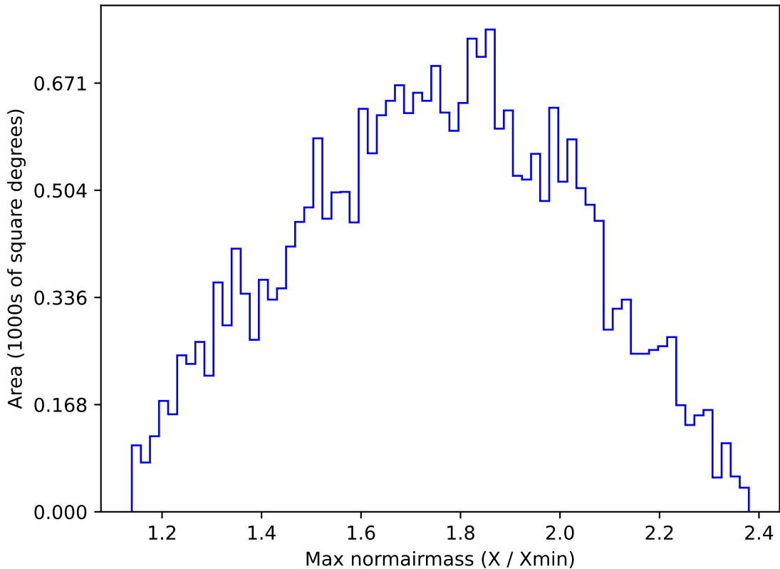
too_elab_r8_d3_ugrizy_v3.4_10yrs All sky g band: Max normairmass
