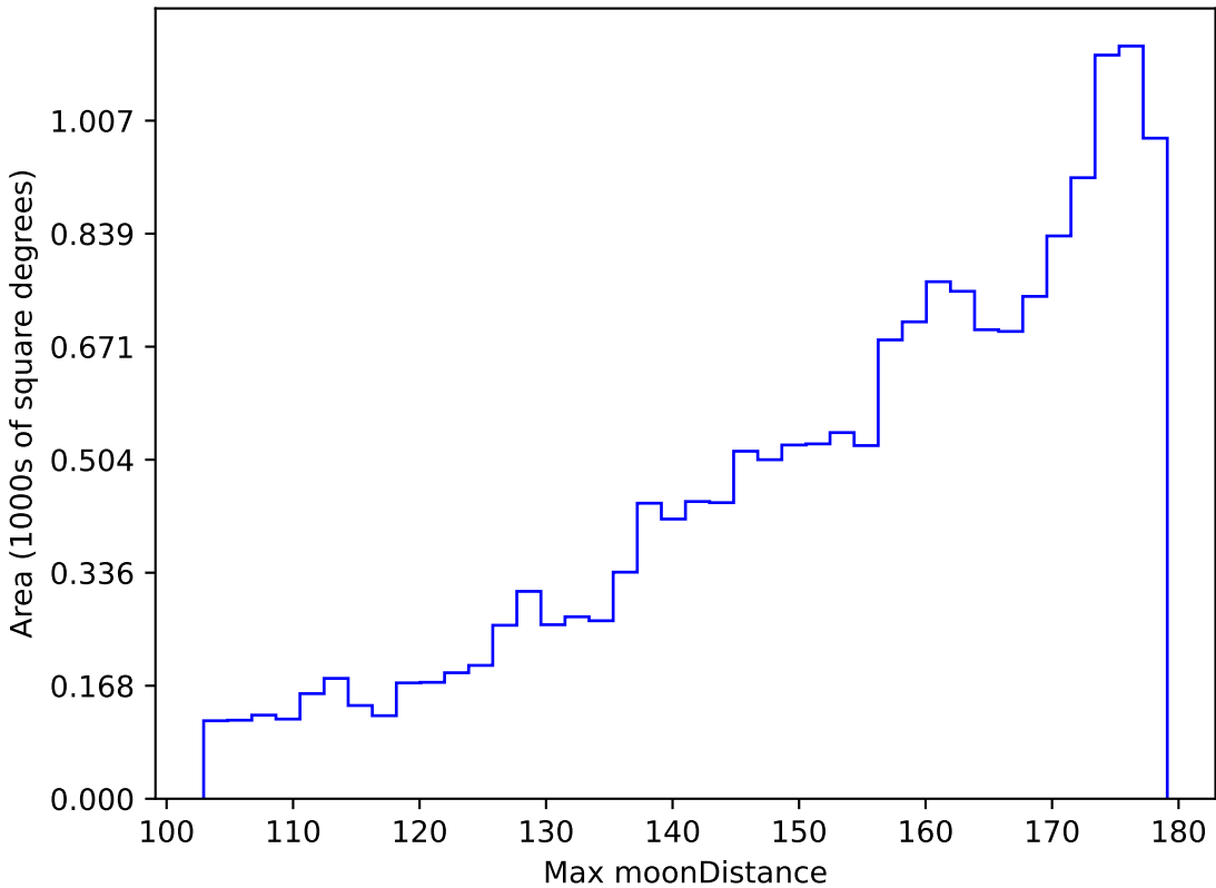
too_elab_r8_d3_ugrizy_v3.4_10yrs WFD z band: Max moonDistance
