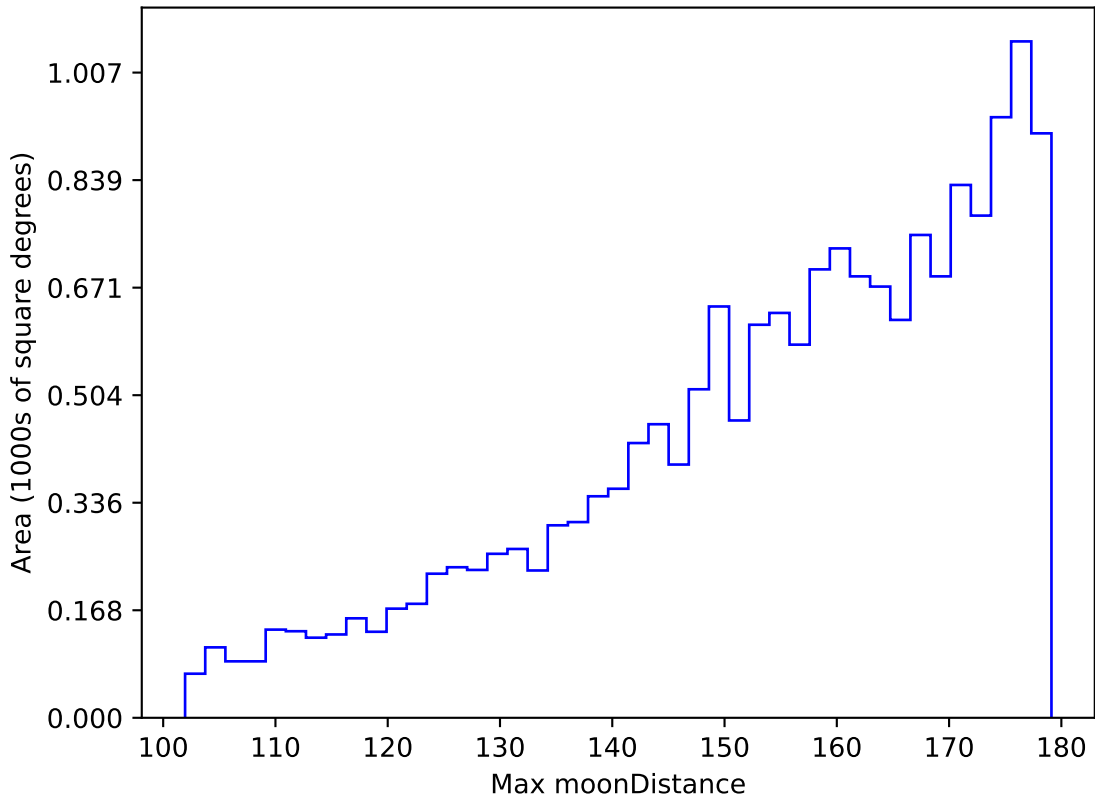
too_elab_r8_d3_ugrizy_v3.4_10yrs WFD u band: Max moonDistance
