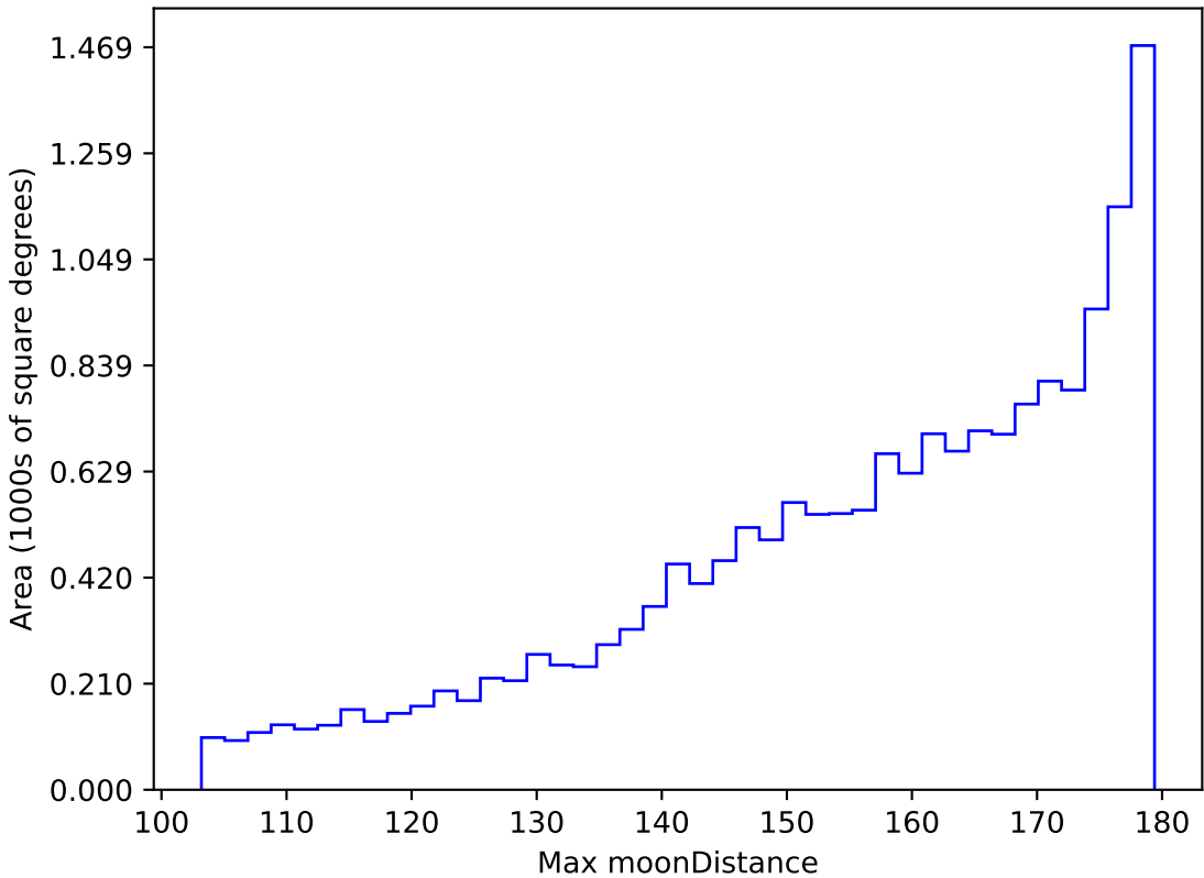
too_elab_r8_d3_ugrizy_v3.4_10yrs WFD r band: Max moonDistance
