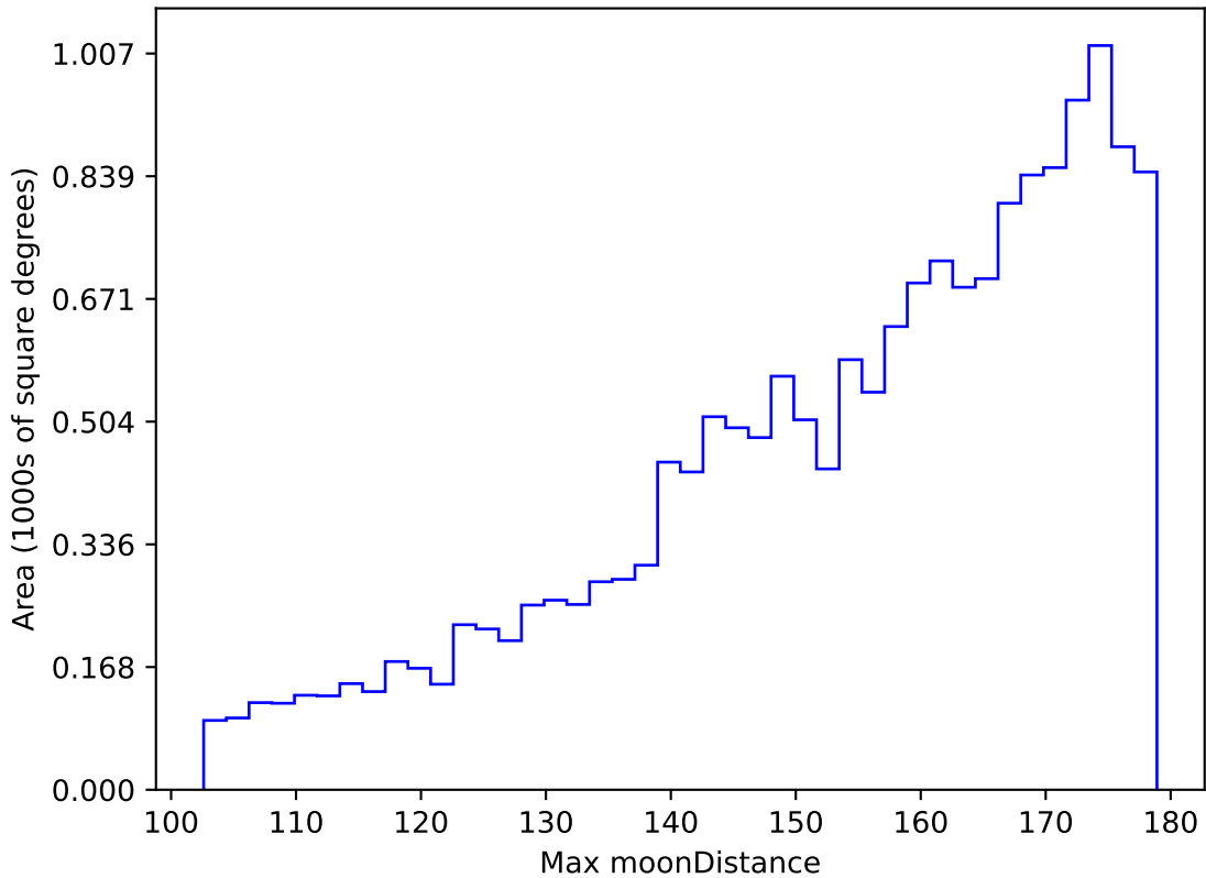
too_elab_r8_d3_ugrizy_v3.4_10yrs WFD g band: Max moonDistance
