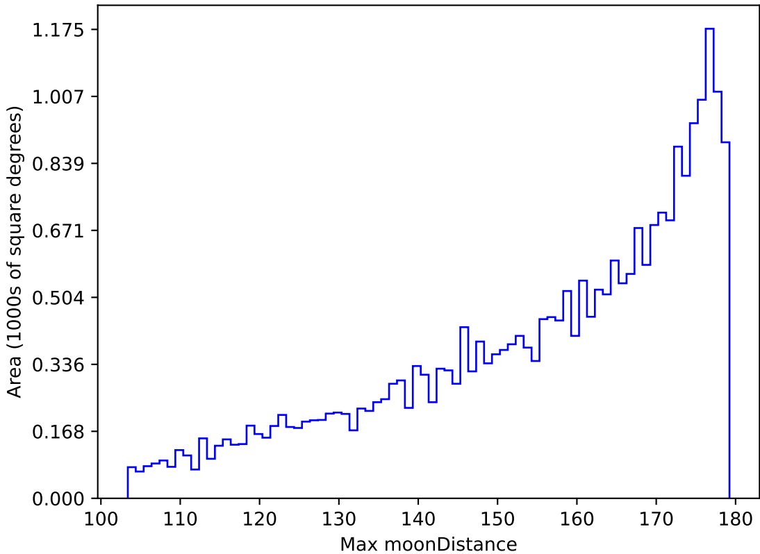
too_elab_r8_d3_ugrizy_v3.4_10yrs All sky i band: Max moonDistance
