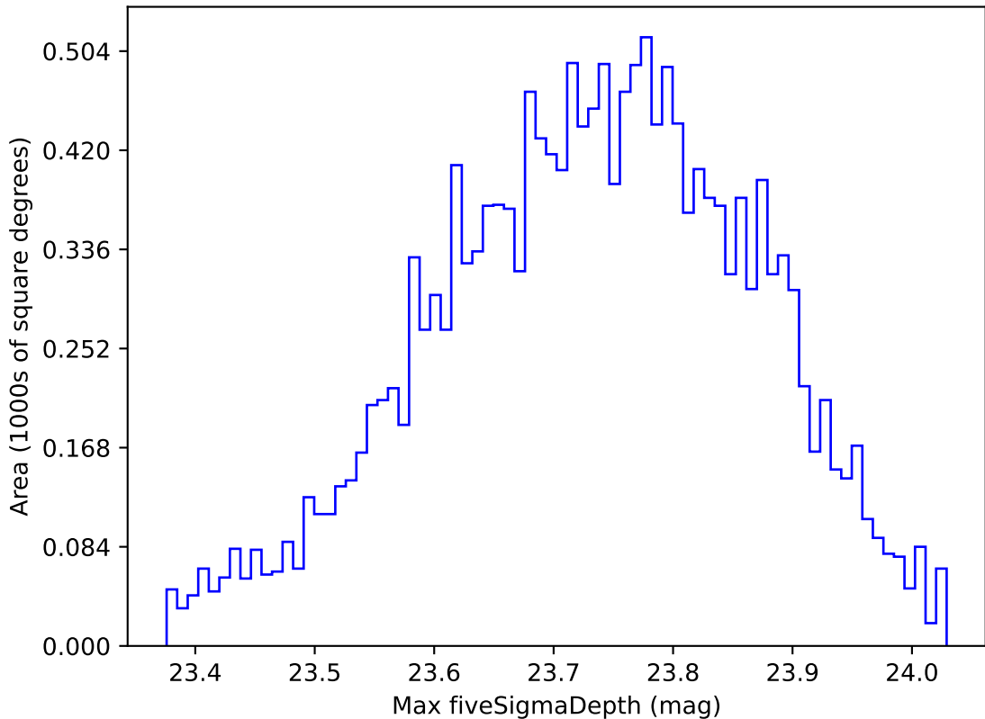
too_elab_r8_d3_ugrizy_v3.4_10yrs WFD u band: Max fiveSigmaDepth
