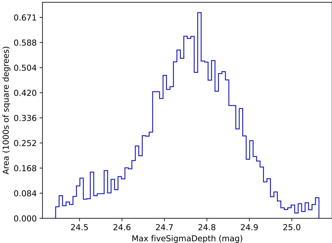
too_elab_r8_d3_ugrizy_v3.4_10yrs WFD r band: Max fiveSigmaDepth
