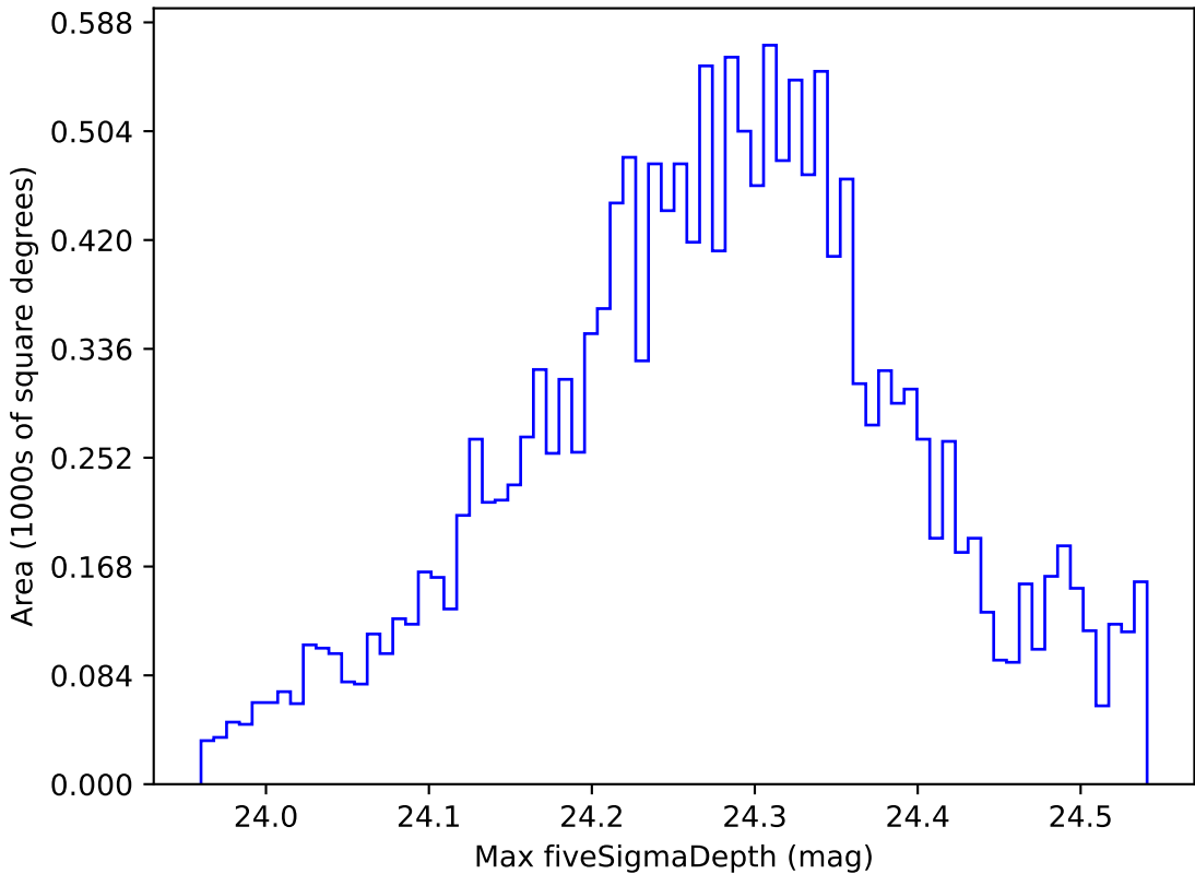
too_elab_r8_d3_ugrizy_v3.4_10yrs WFD i band: Max fiveSigmaDepth
