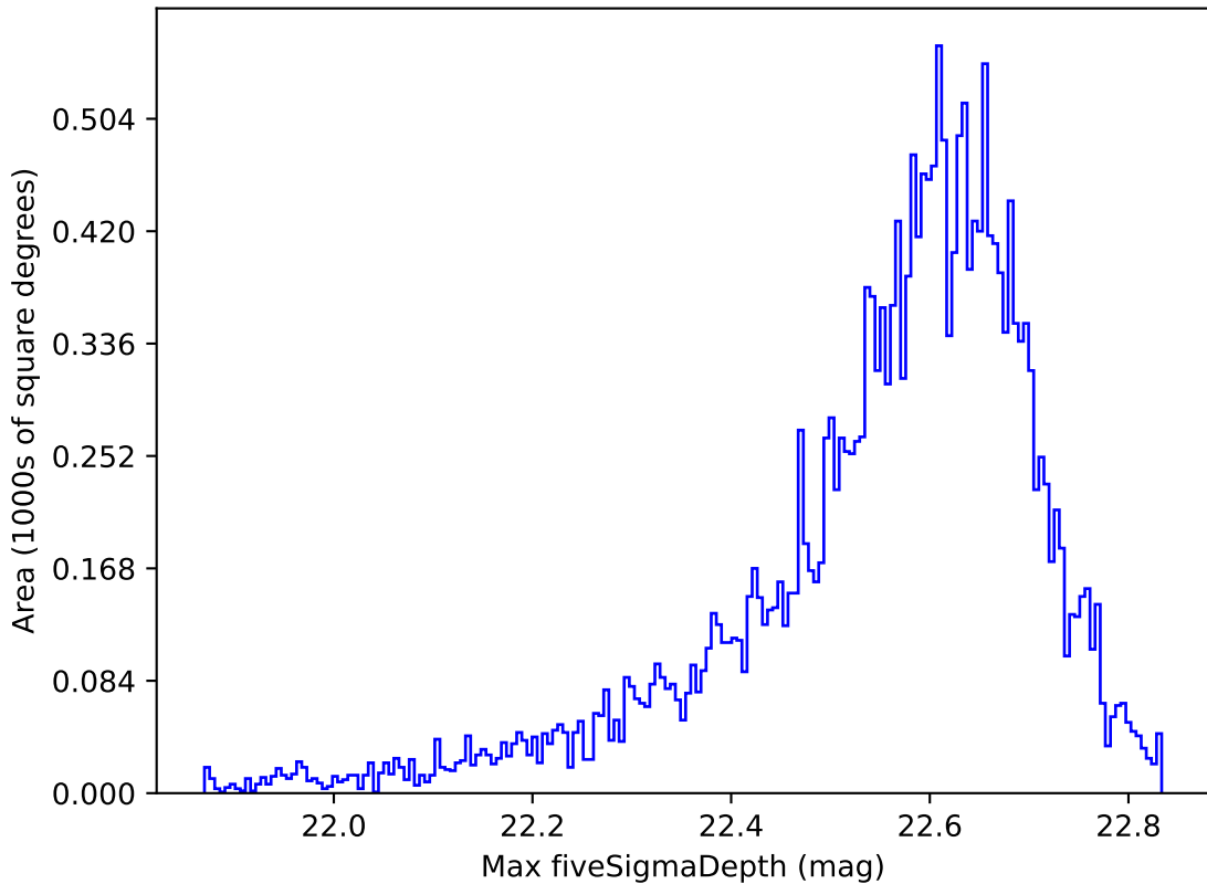
too_elab_r8_d3_ugrizy_v3.4_10yrs All sky y band: Max fiveSigmaDepth
