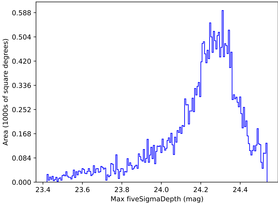
too_elab_r8_d3_ugrizy_v3.4_10yrs All sky i band: Max fiveSigmaDepth
