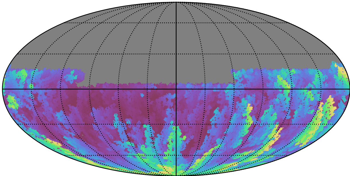
too_elab_r8_d3_ugrizy_v3.4_10yrs Yr 1 u band: Max airmass
