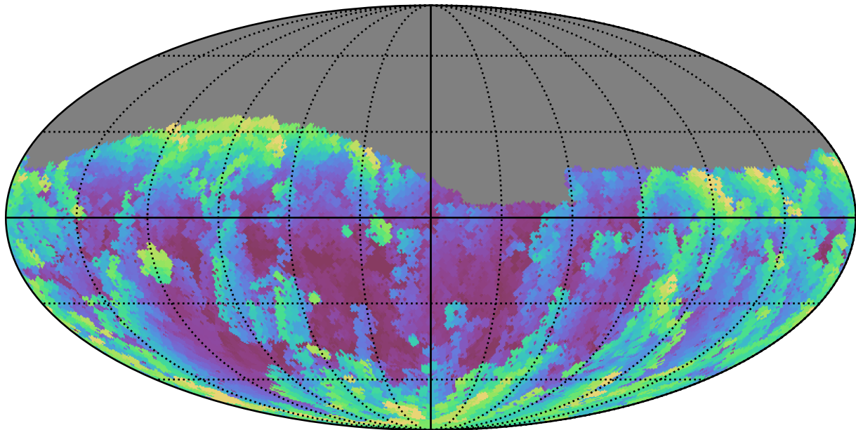
too_elab_r8_d3_ugrizy_v3.4_10yrs Yr 1 g band: Max airmass
