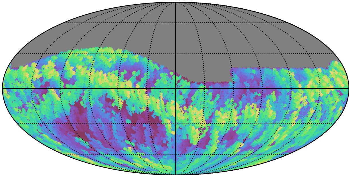
too_elab_r8_d3_ugrizy_v3.4_10yrs Yr 1 all bands: Max airmass
