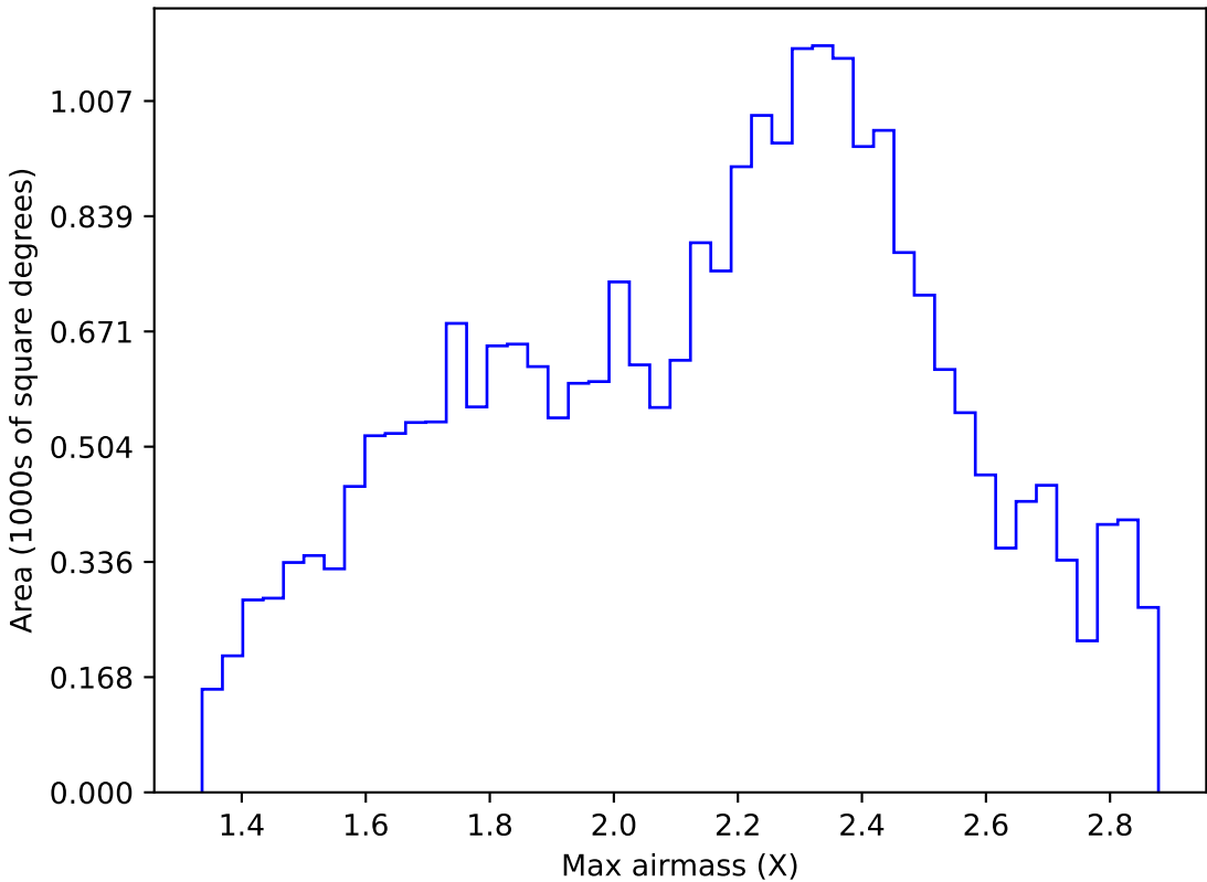
too_elab_r8_d3_ugrizy_v3.4_10yrs Yr 1 all bands: Max airmass
