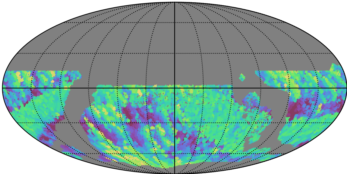
too_elab_r8_d3_ugrizy_v3.4_10yrs WFD r band: Max airmass
