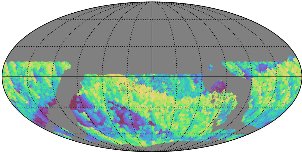
too_elab_r8_d3_ugrizy_v3.4_10yrs WFD i band: Max airmass
