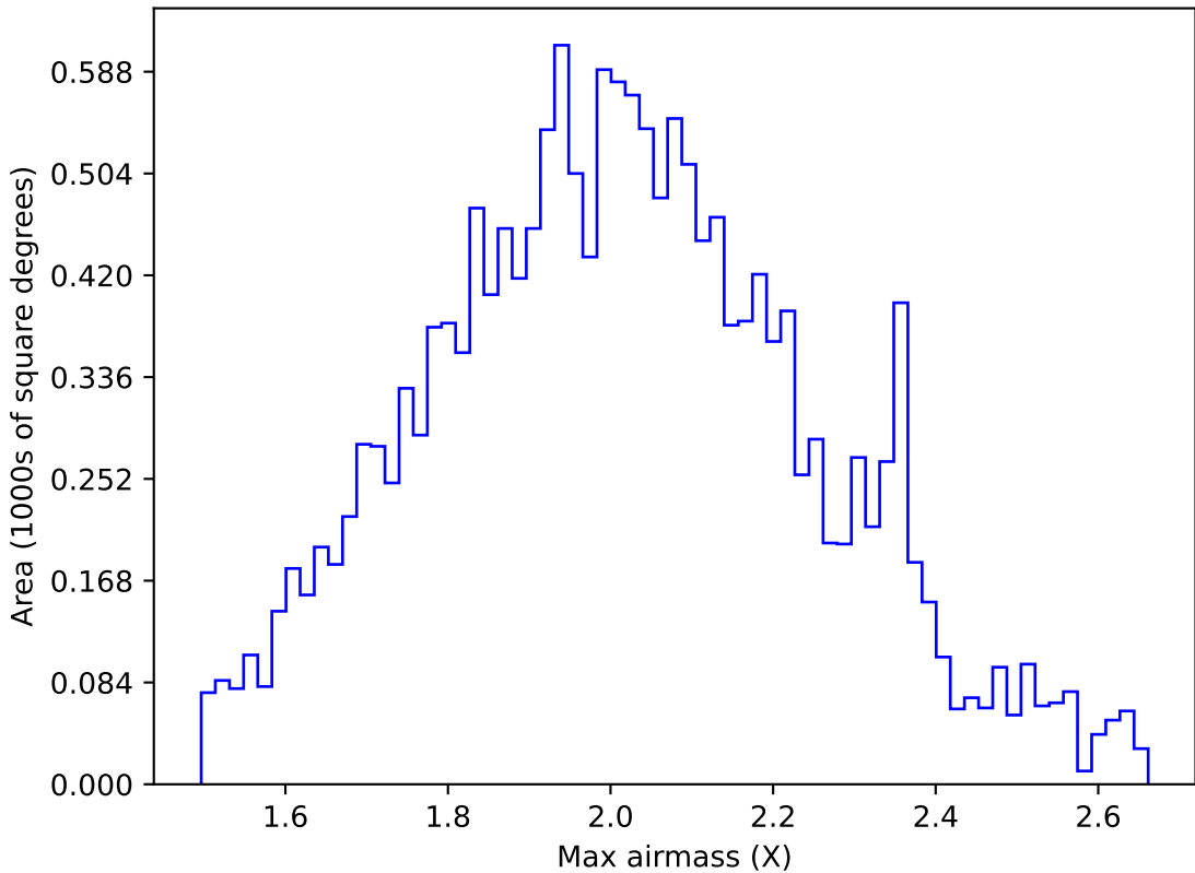
too_elab_r8_d3_ugrizy_v3.4_10yrs WFD g band: Max airmass
