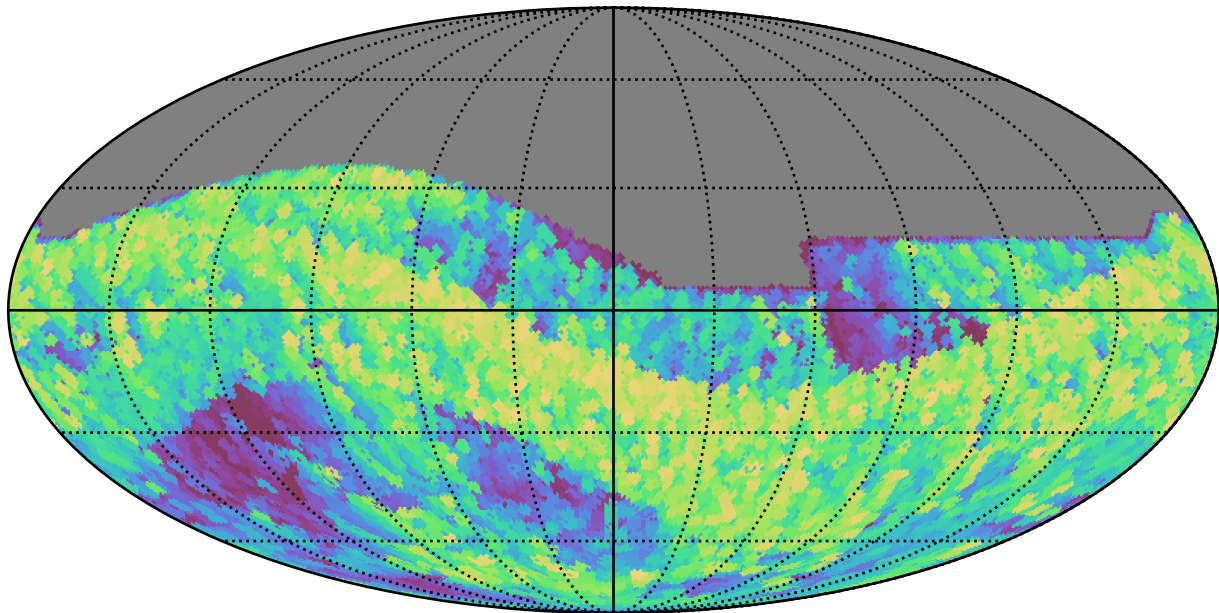
too_elab_r8_d3_ugrizy_v3.4_10yrs All sky z band: Max airmass
