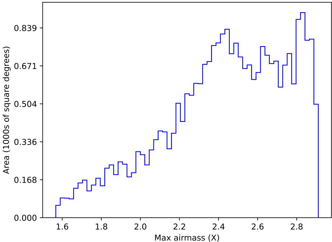
too_elab_r8_d3_ugrizy_v3.4_10yrs All sky z band: Max airmass
