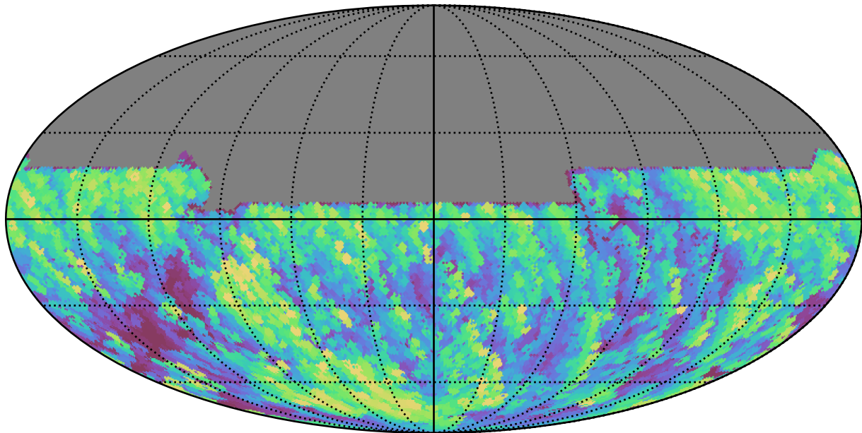
too_elab_r8_d3_ugrizy_v3.4_10yrs All sky y band: Max airmass
