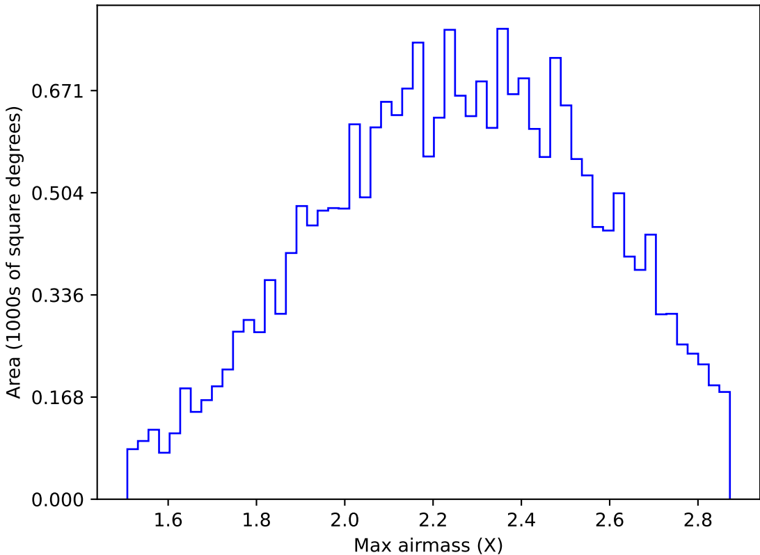
too_elab_r8_d3_ugrizy_v3.4_10yrs All sky y band: Max airmass
