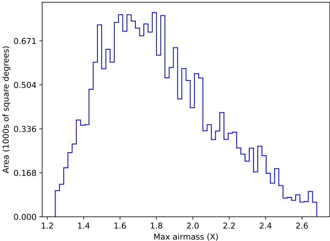
too_elab_r8_d3_ugrizy_v3.4_10yrs All sky u band: Max airmass
