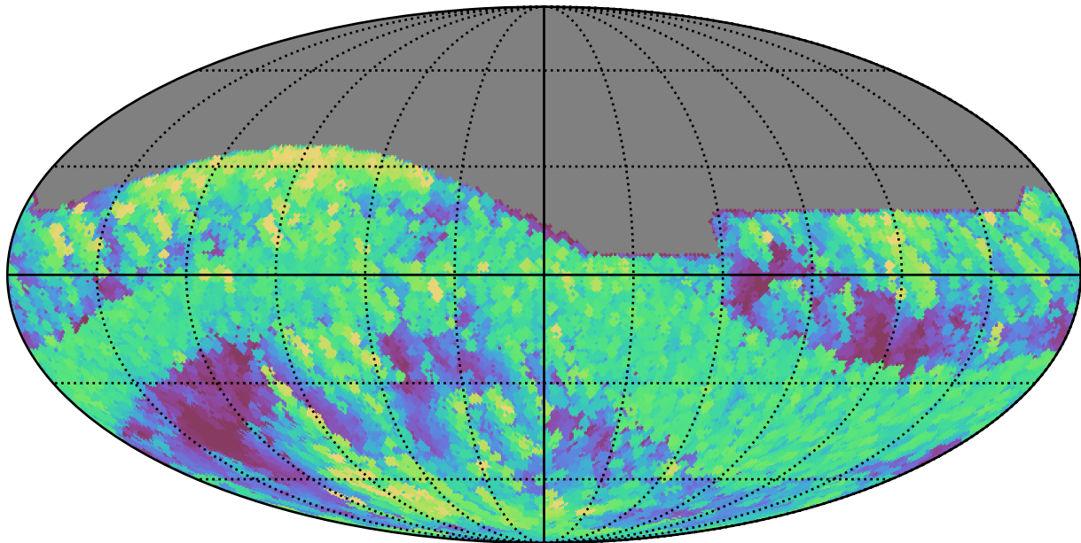
too_elab_r8_d3_ugrizy_v3.4_10yrs All sky r band: Max airmass
