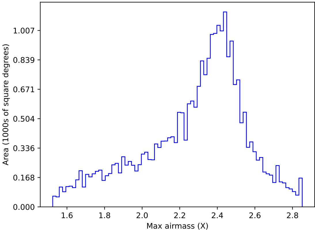
too_elab_r8_d3_ugrizy_v3.4_10yrs All sky r band: Max airmass
