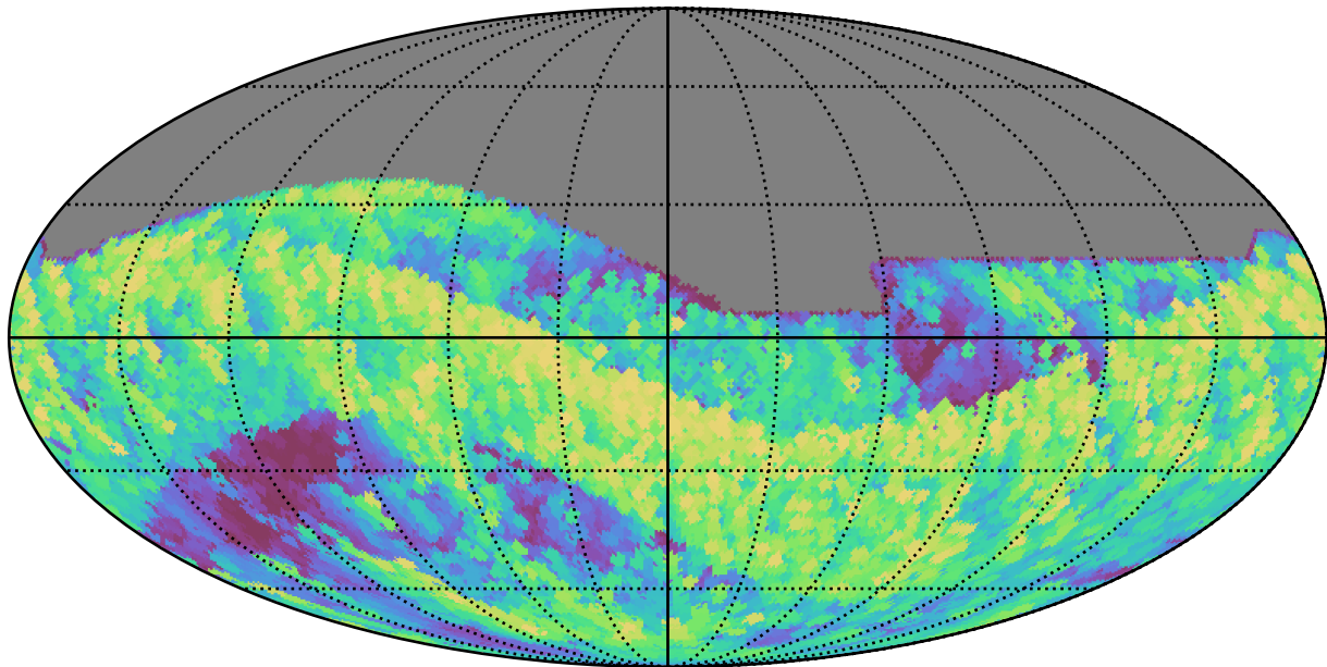
too_elab_r8_d3_ugrizy_v3.4_10yrs All sky i band: Max airmass
