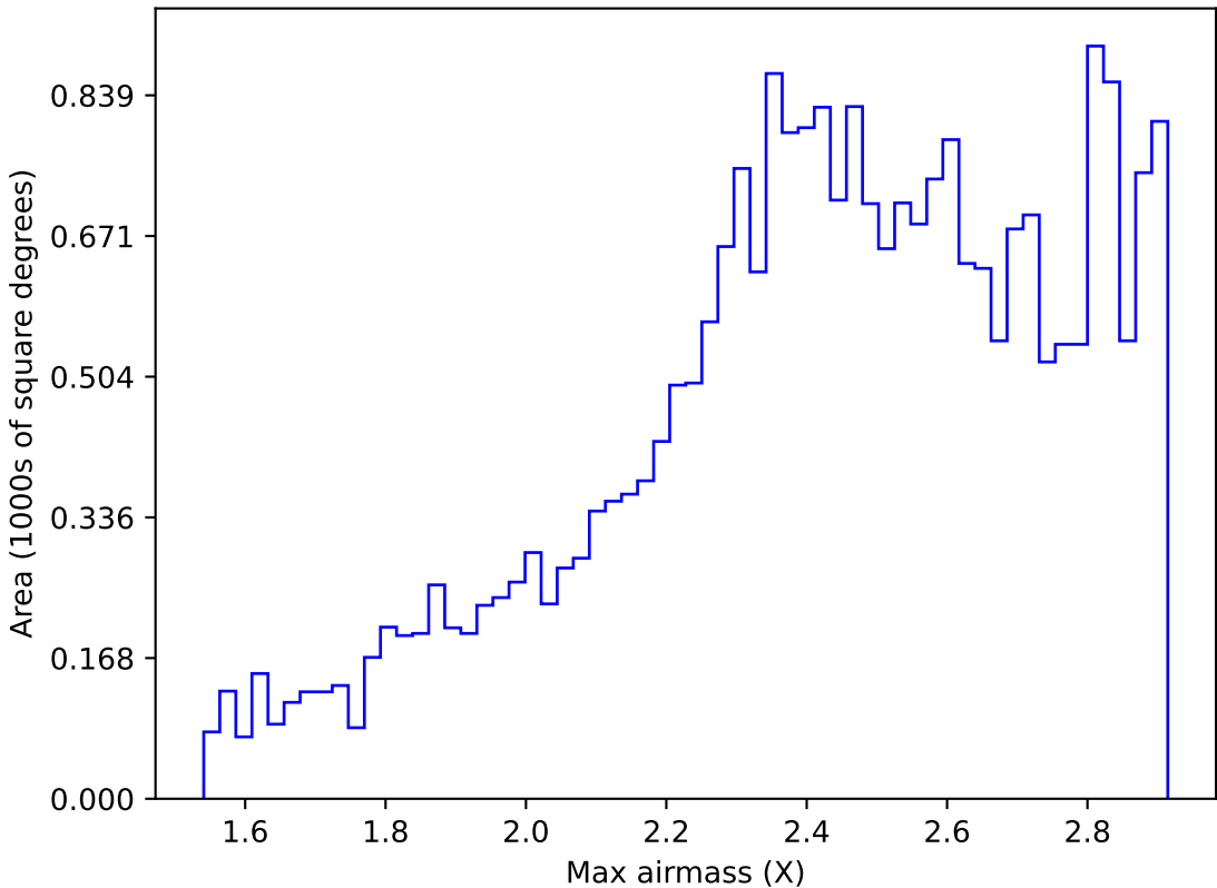
too_elab_r8_d3_ugrizy_v3.4_10yrs All sky i band: Max airmass
