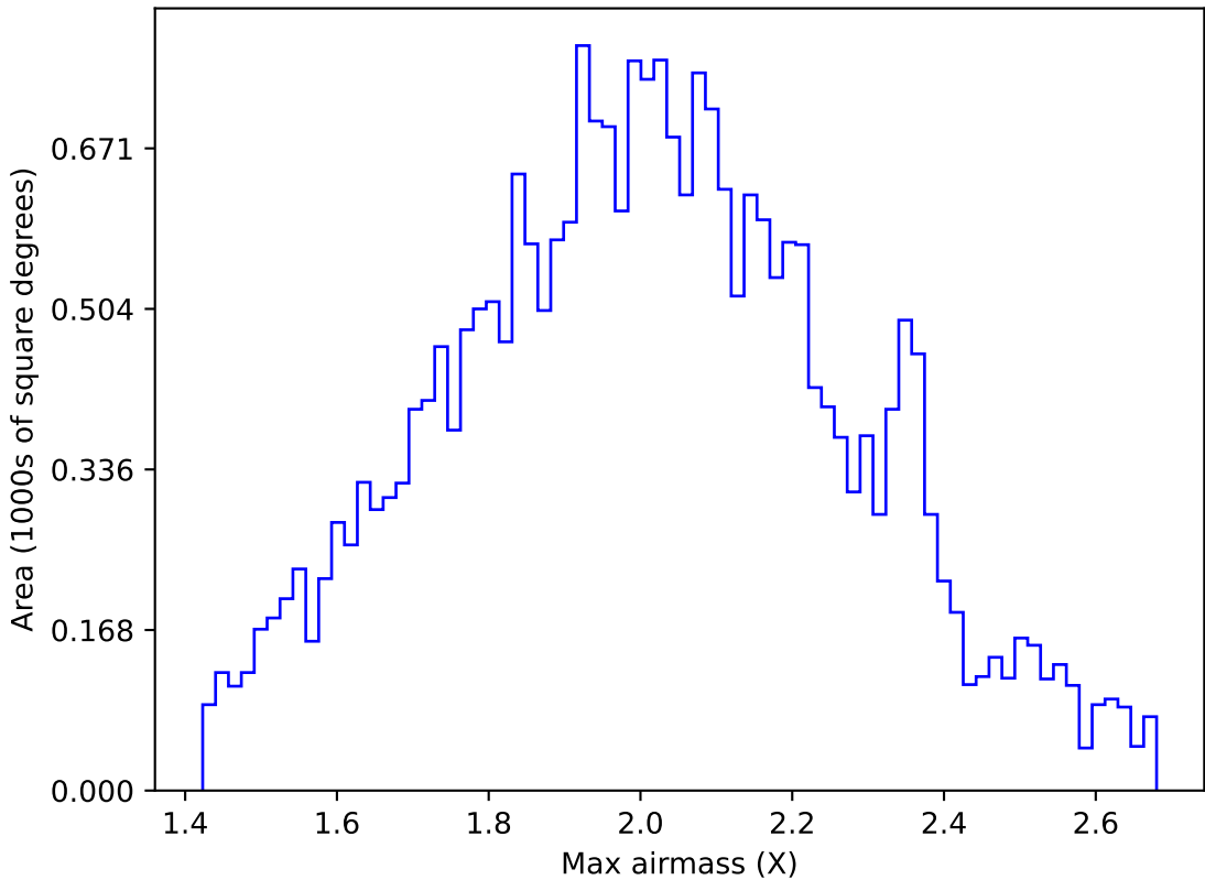
too_elab_r8_d3_ugrizy_v3.4_10yrs All sky g band: Max airmass
