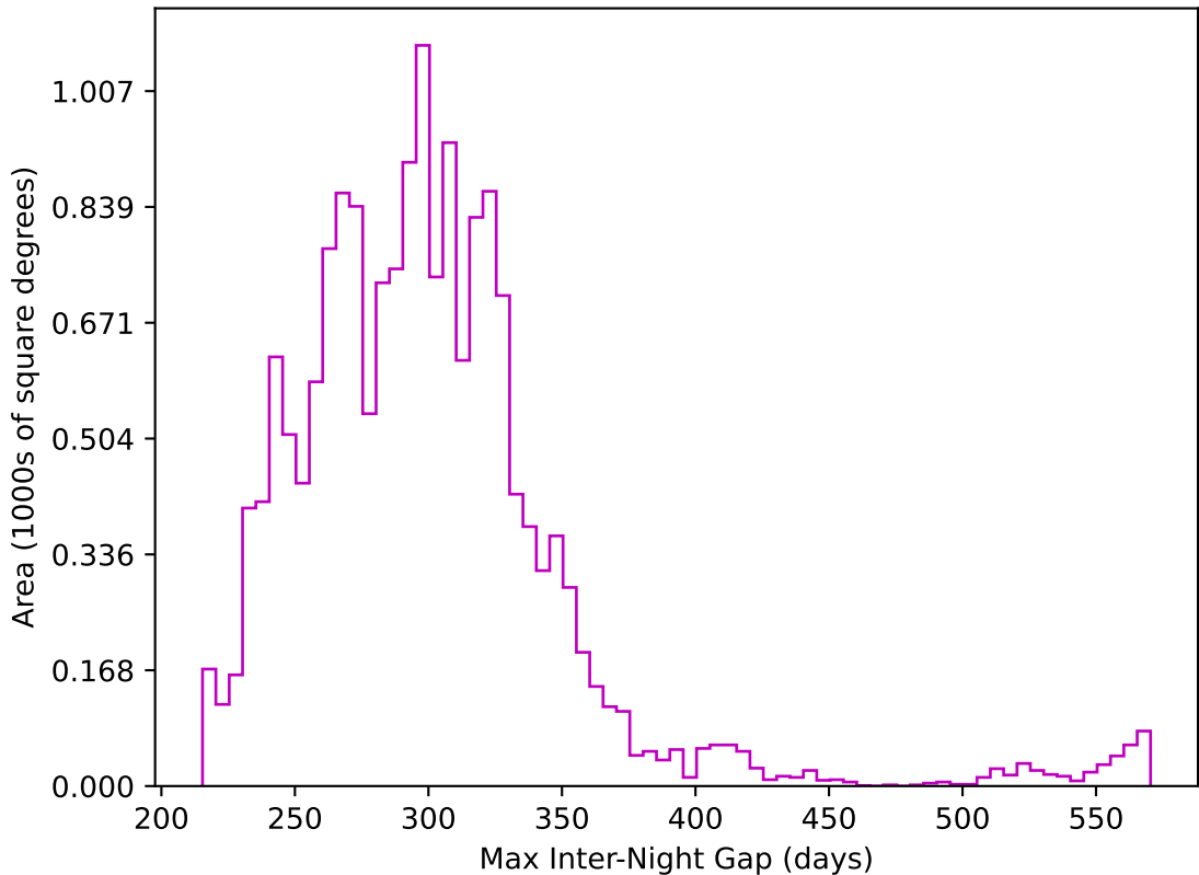
too_elab_r8_d3_ugrizy_v3.4_10yrs WFD z band: Max Inter-Night Gap
