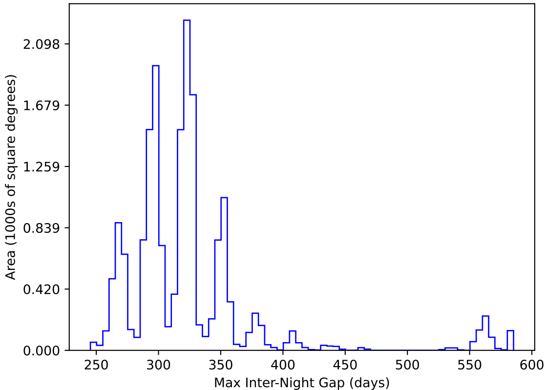
too_elab_r8_d3_ugrizy_v3.4_10yrs WFD y band: Max Inter-Night Gap
