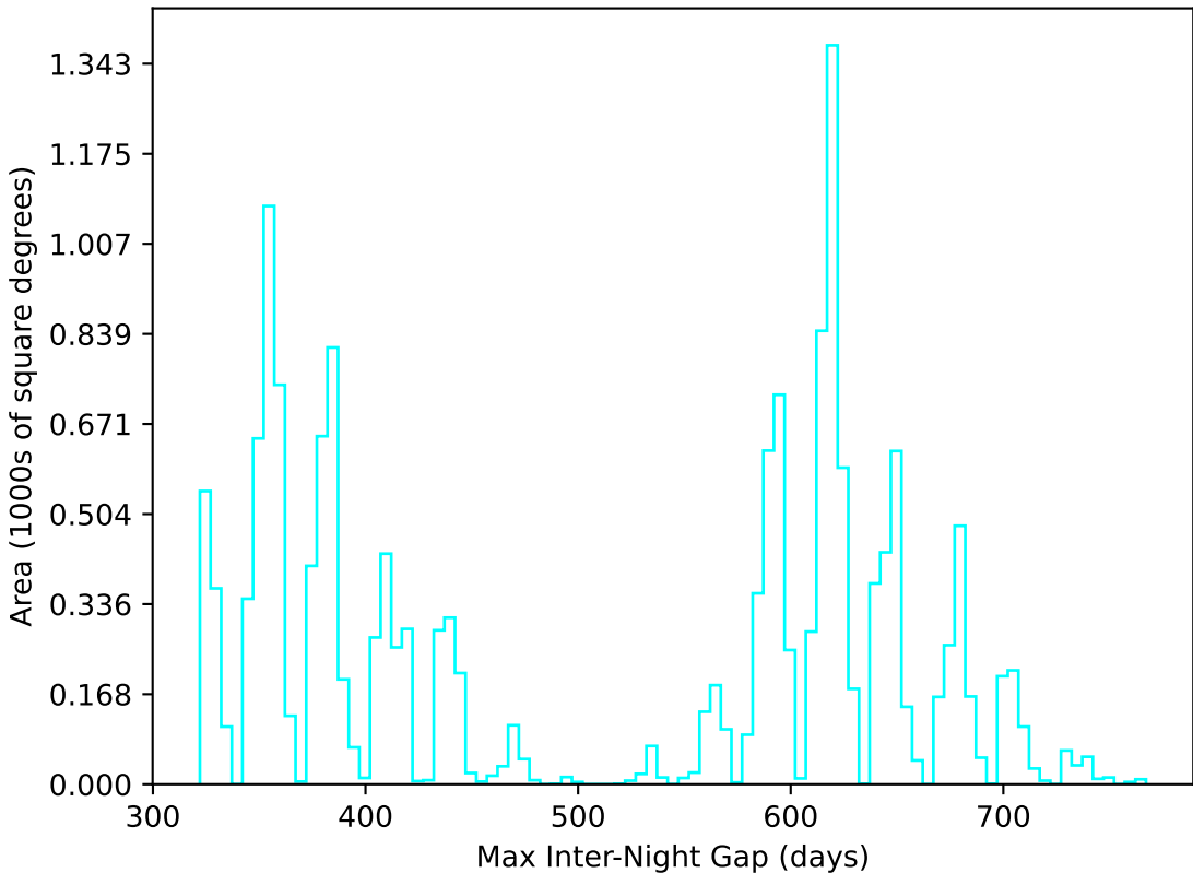
too_elab_r8_d3_ugrizy_v3.4_10yrs WFD u band: Max Inter-Night Gap
