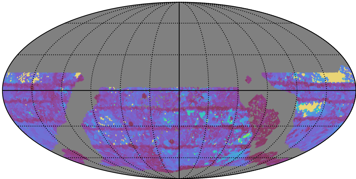
too_elab_r8_d3_ugrizy_v3.4_10yrs WFD r band: Max Inter-Night Gap
