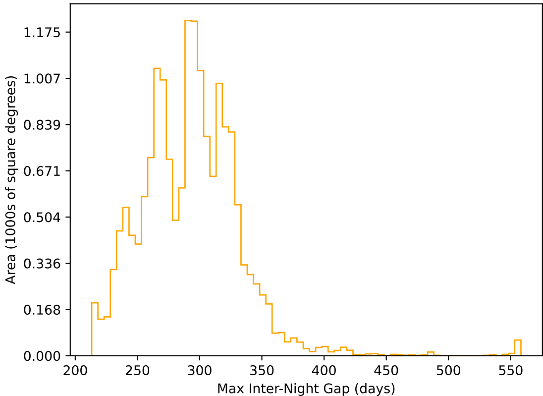
too_elab_r8_d3_ugrizy_v3.4_10yrs WFD r band: Max Inter-Night Gap
