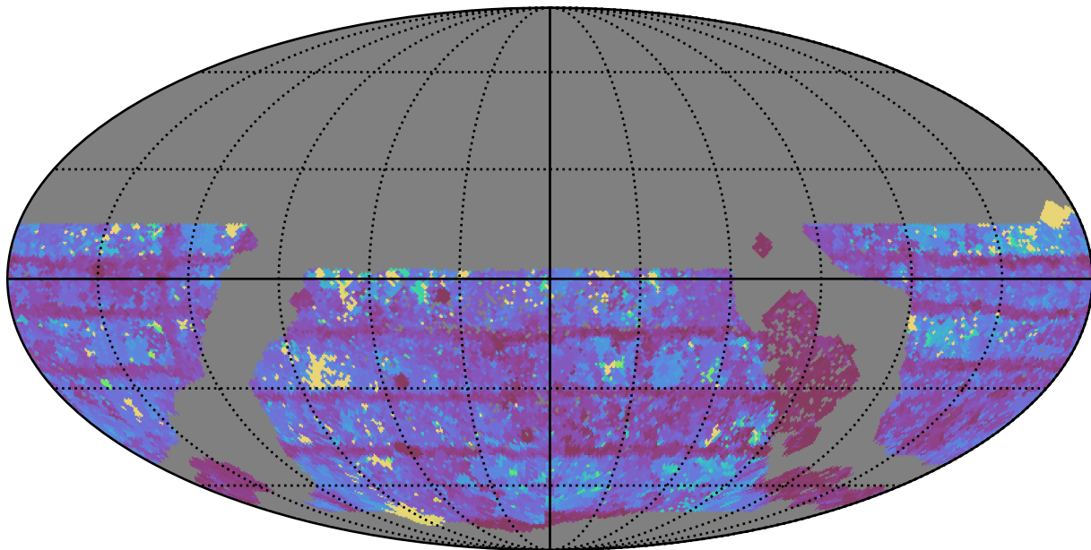
too_elab_r8_d3_ugrizy_v3.4_10yrs WFD i band: Max Inter-Night Gap
