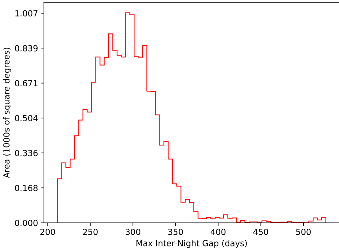
too_elab_r8_d3_ugrizy_v3.4_10yrs WFD i band: Max Inter-Night Gap
